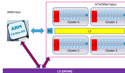
Figure 2.1: Internal Architecture of STHORM MPSoC System
